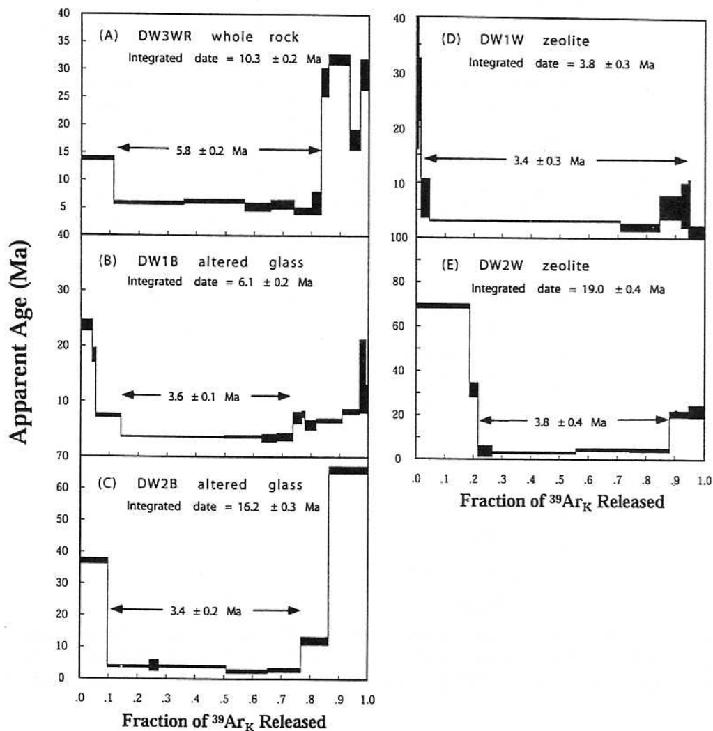
Figure 2. Apparent age spectra for all of the samples analysed. The plateau date is given between the arrows and the arrows cover the gas fractions included into the calculation of the plateau date. The integrated date is given in parentheses below the sample name with the group number for each sample. Boxes for each step extend vertically to \pm 1\sigma , and horizontally in proportion to the fraction of ^{39}\text{Ar} released in the step.
