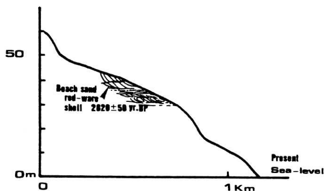
Figure 6. The marine terrace in the Heifachiao area, about 25-40 m in altitude, is composed of well-sorted sands and many of shell-debris and red-ware chips.
