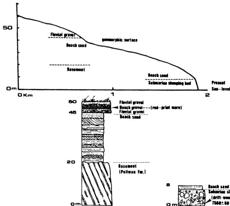
Figure 7. The marine terrace in the Yuchia area, about 8-45 m in altitude, is composed of well-sorted marine sands. A part of basement of the marine terrace is a submarine slumping bed which consists of poorly-sorted sands/gravels, shell-debris and drift-wood.
